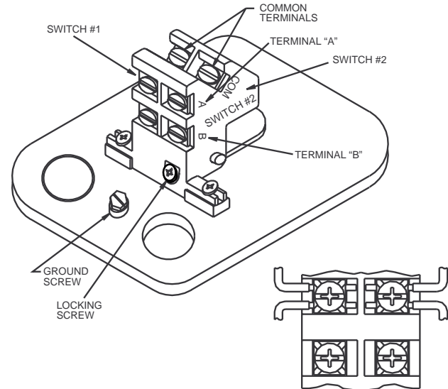
Figure 3. Switch terminals:
